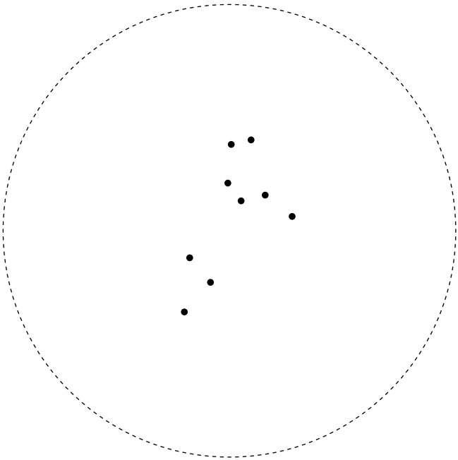
Leo
