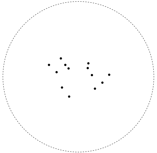
Phoenix
