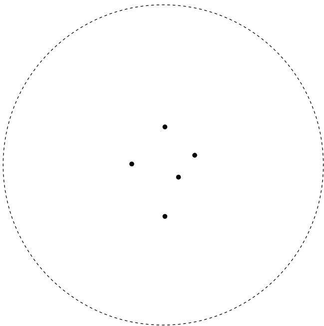
Southern Cross
