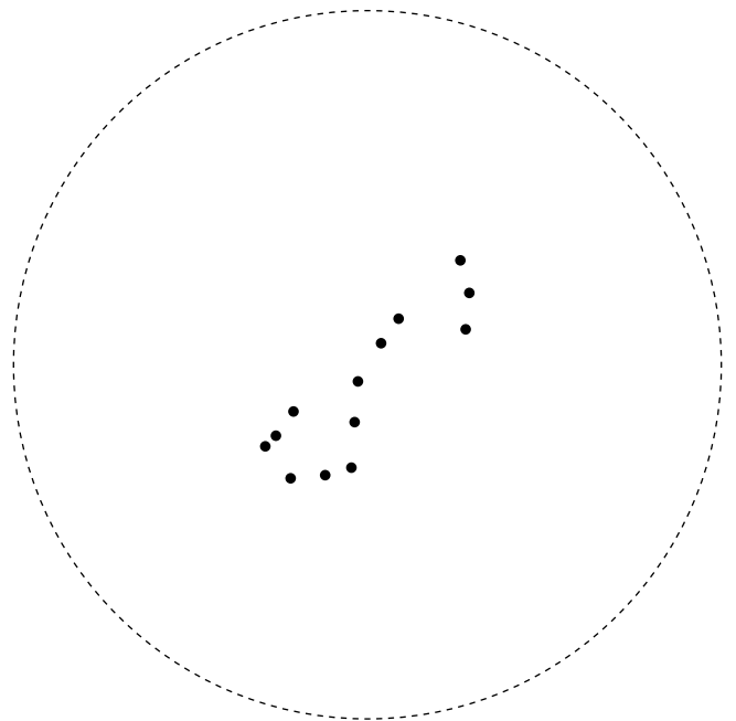
Scorpius
